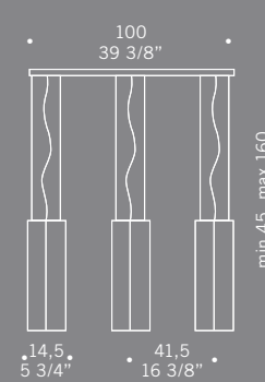
CARRÈ S3PL 3x70W E27 alogeno chiara clear halogen 3x26W E27 fluorescente fluorescent
