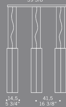
CARRÈ S3GL 3x70W E27 alogeno chiara clear halogen 3x26W E27 fluorescente fluorescent
